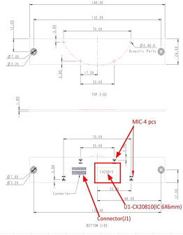
MIC Board-Curve Shape
