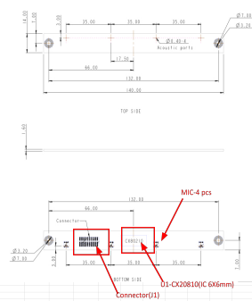
MIC Board-Straight Line
