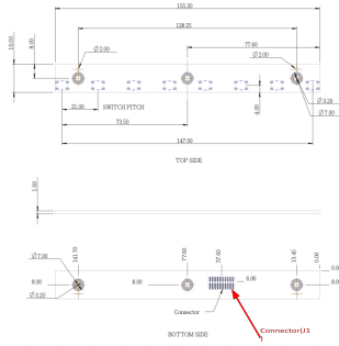
MIC Board-Straight Line
