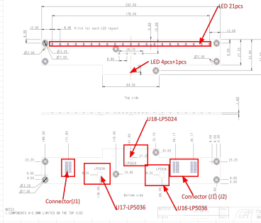
MIC Board-Curve Shape
