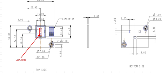
LED Side Board
